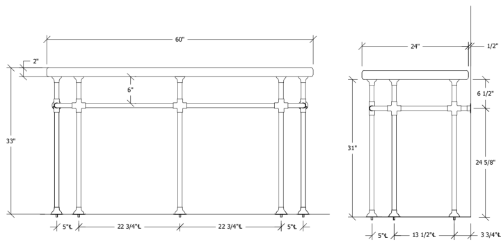
UA2831-7 SL Modern Industrial Outer Curved Base 7 Legs
