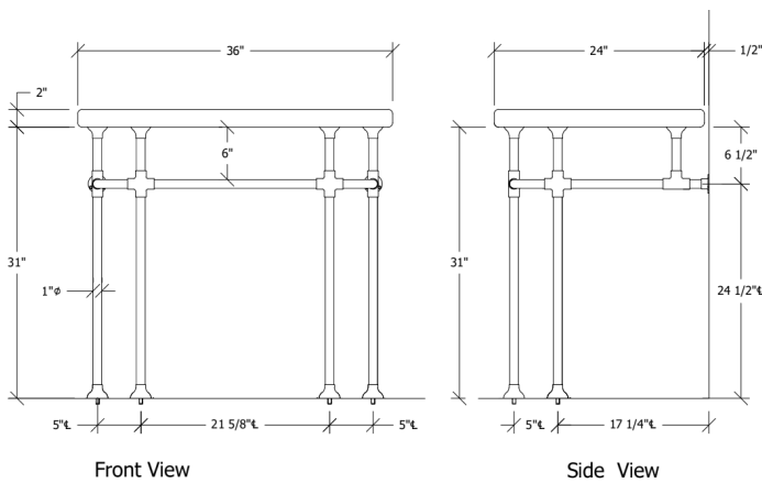
UA2831-4 SL Modern Industrial Outer Curved Base 4 Legs
