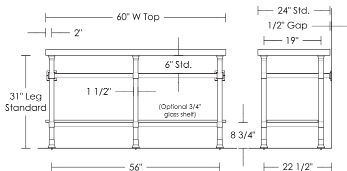
UA2819-B SL 5 Legs with 5 Lower Bars
