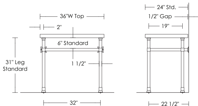
UA2817 SL 4 Leg Base
