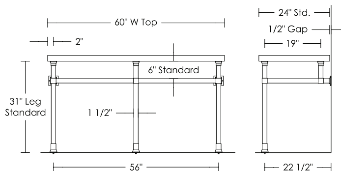
UA2816 SL 3 Leg Base
