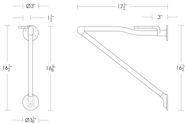
Typical Installation
