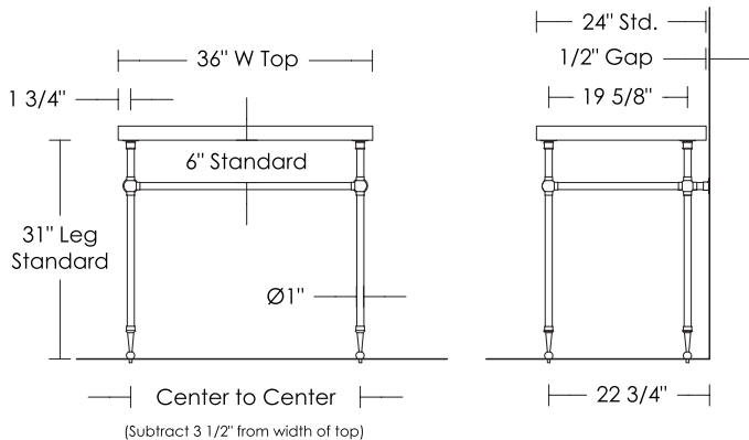
UA2743 SL 4 Legs [1"Ø] with Mott Cap & Foot
