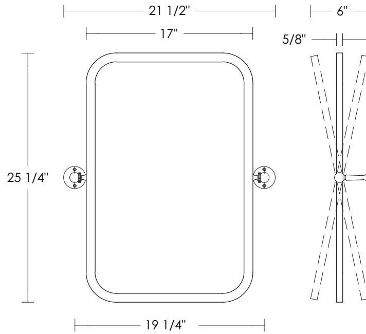
Pivoting Mirror with Round Brackets – Vertical
