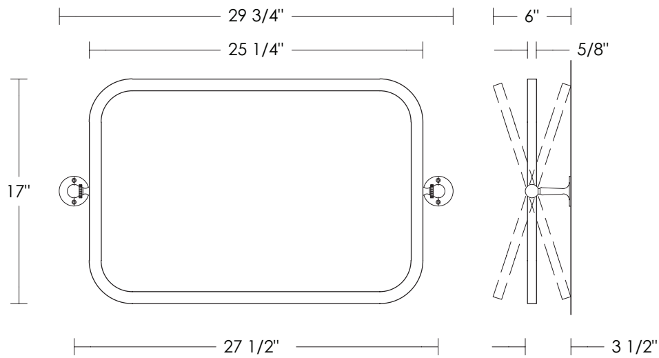
Pivoting Mirror with Round Brackets – Horizontal
