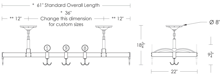
UA5016-PM Pot Rack without Lights
