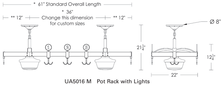
UA5016 M Pot Rack with Lights
