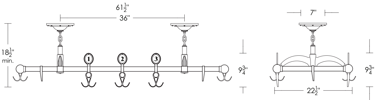
UA5016-P M Industrial Pot Rack without Lights
