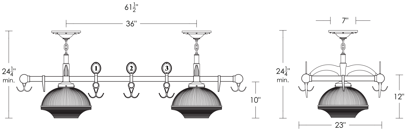
UA5016-PS M Industrial Pot Rack with Lights
